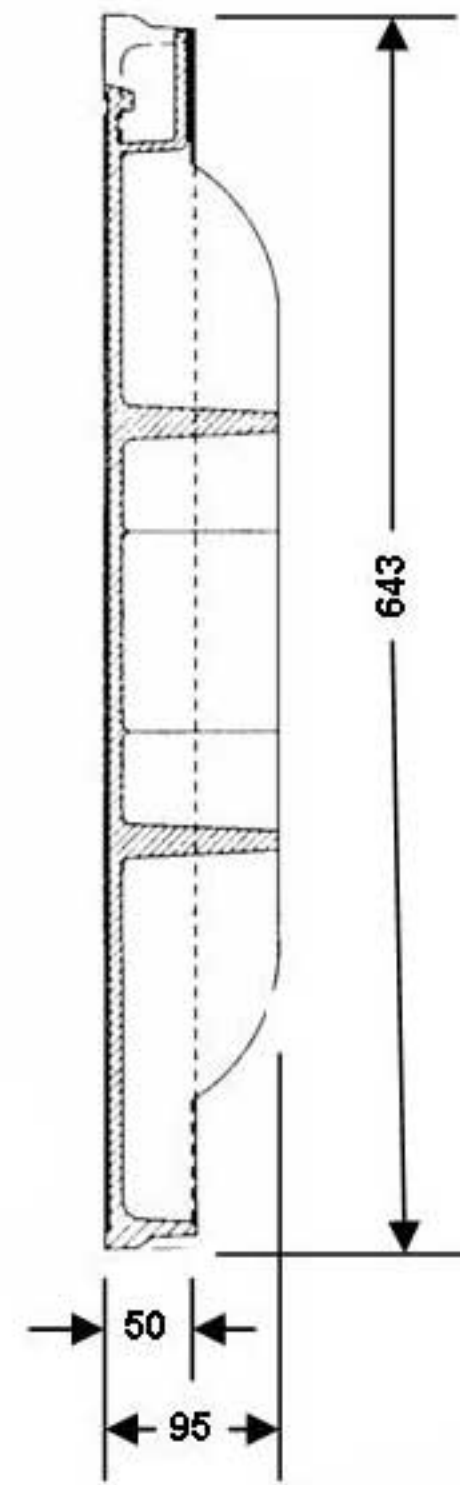
SECTION 'A-A'
