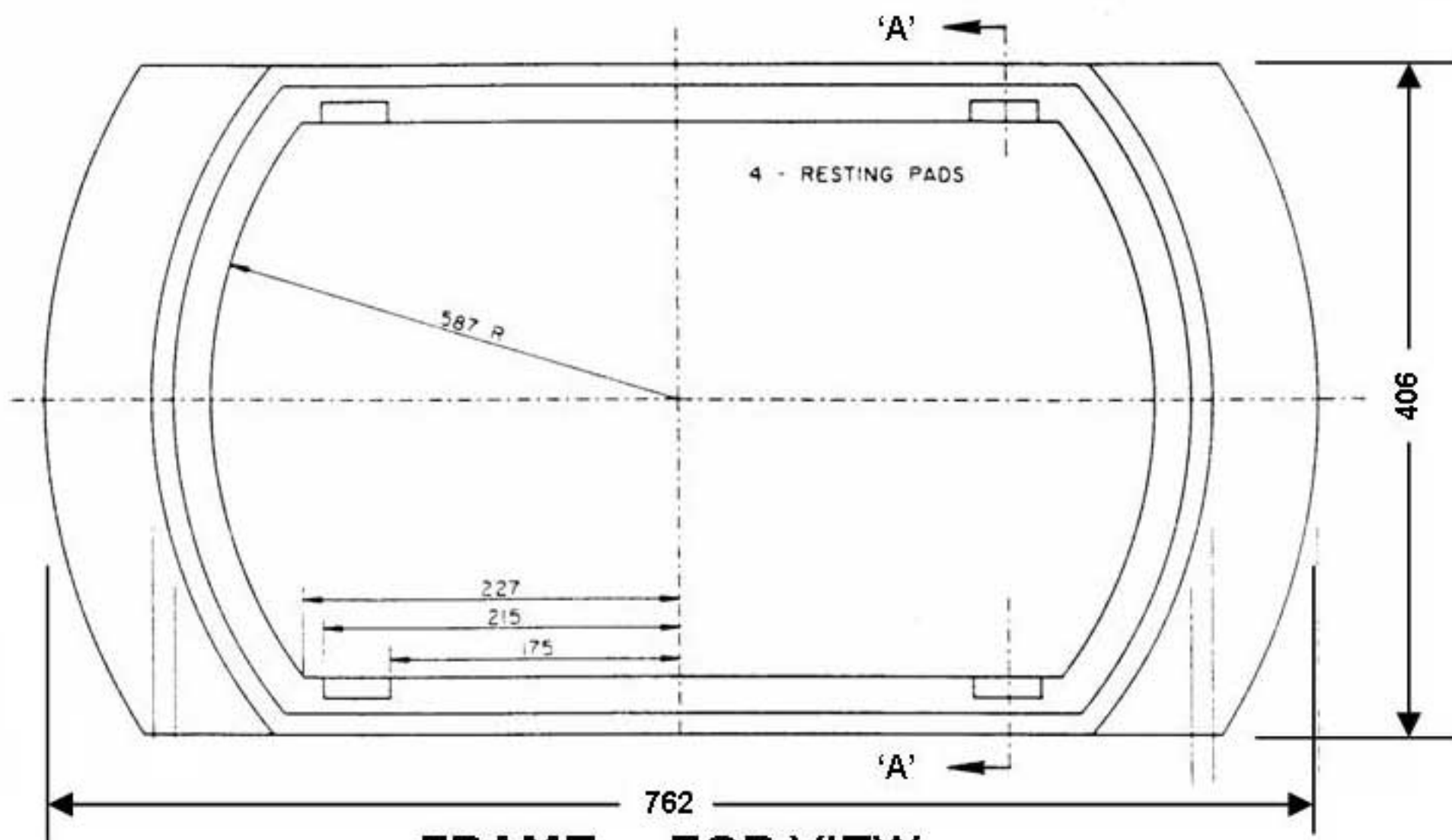
FRAME - TOP VIEW
