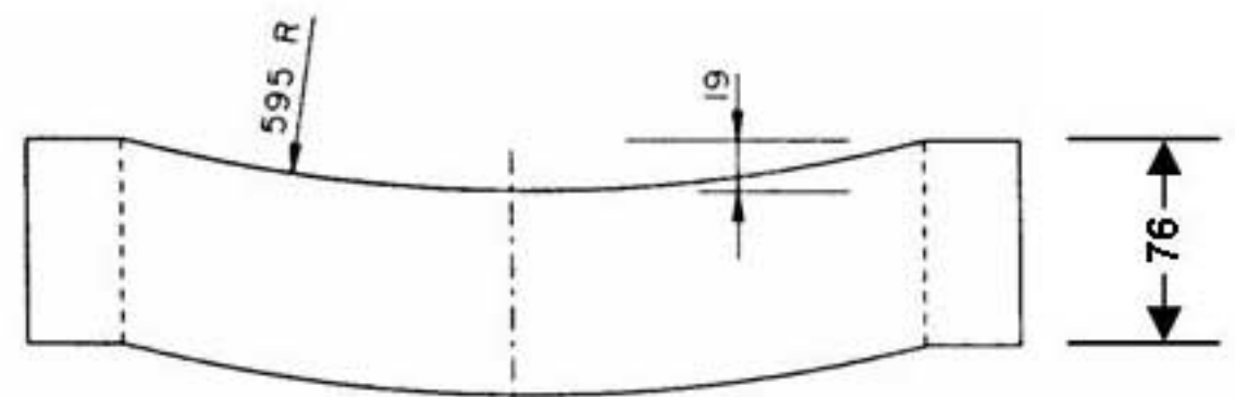
GRATE - END VIEW
