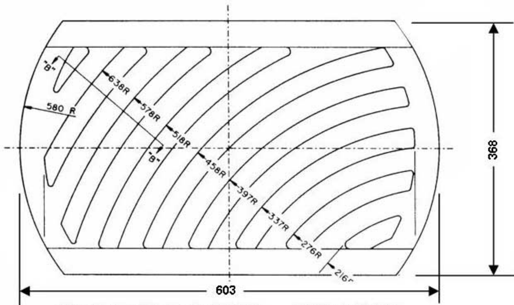
GRATE (LEFT HAND) - TOP VIEW
