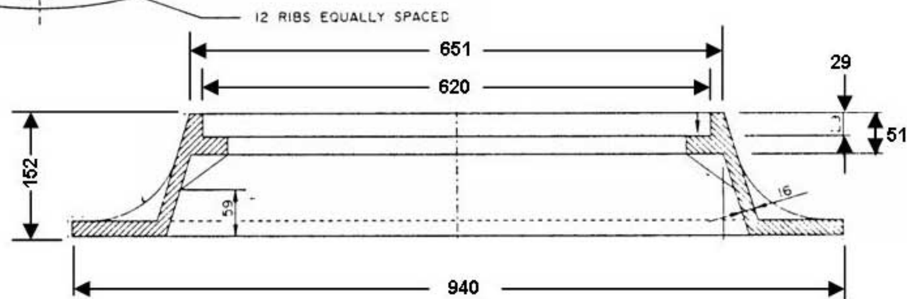
6" FRAME SECTION 'A-A'
