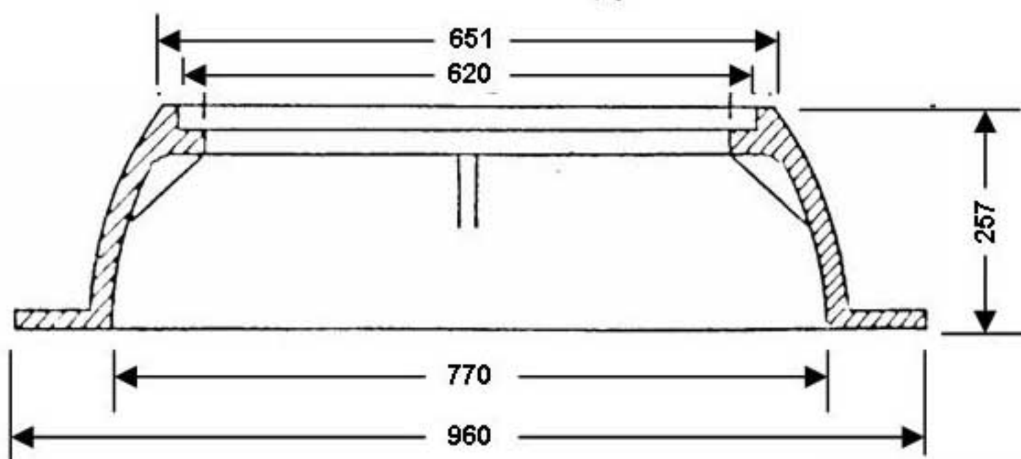
10" FRAME - CROSS SECTION
