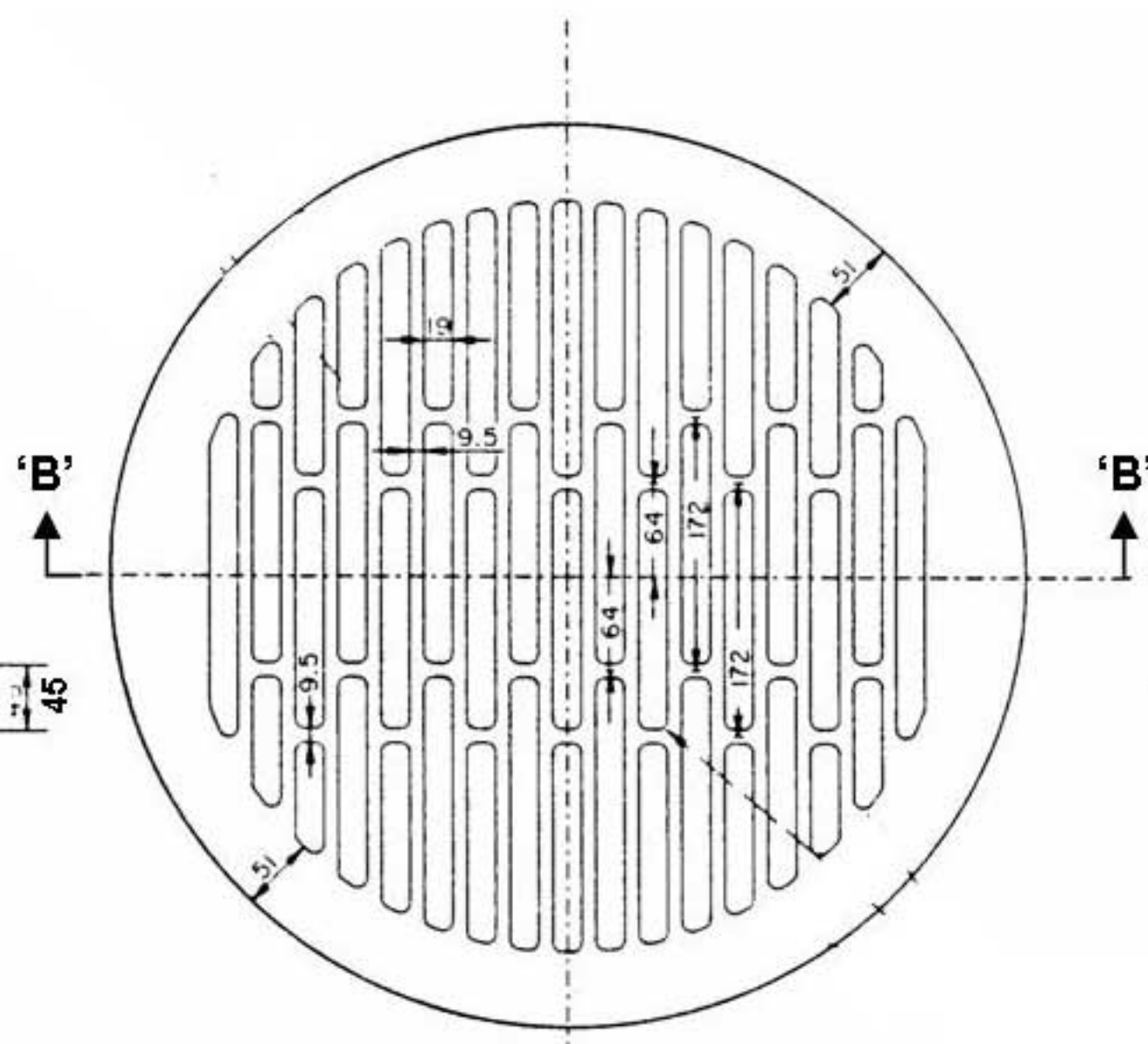
GRATE - TOP VIEW
