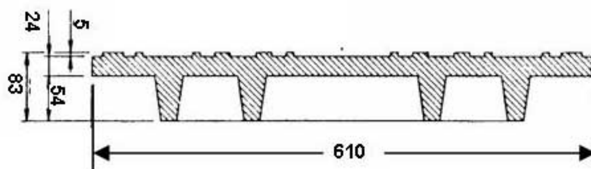
COVER - SECTION 'A-A'
