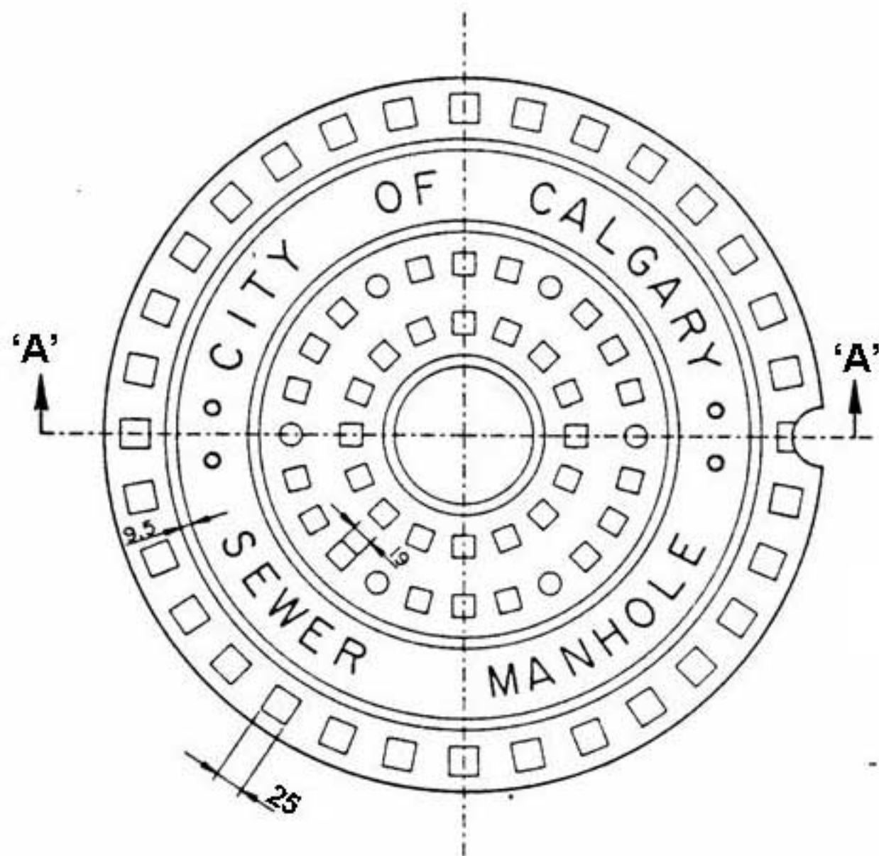
COVER - TOP VIEW
