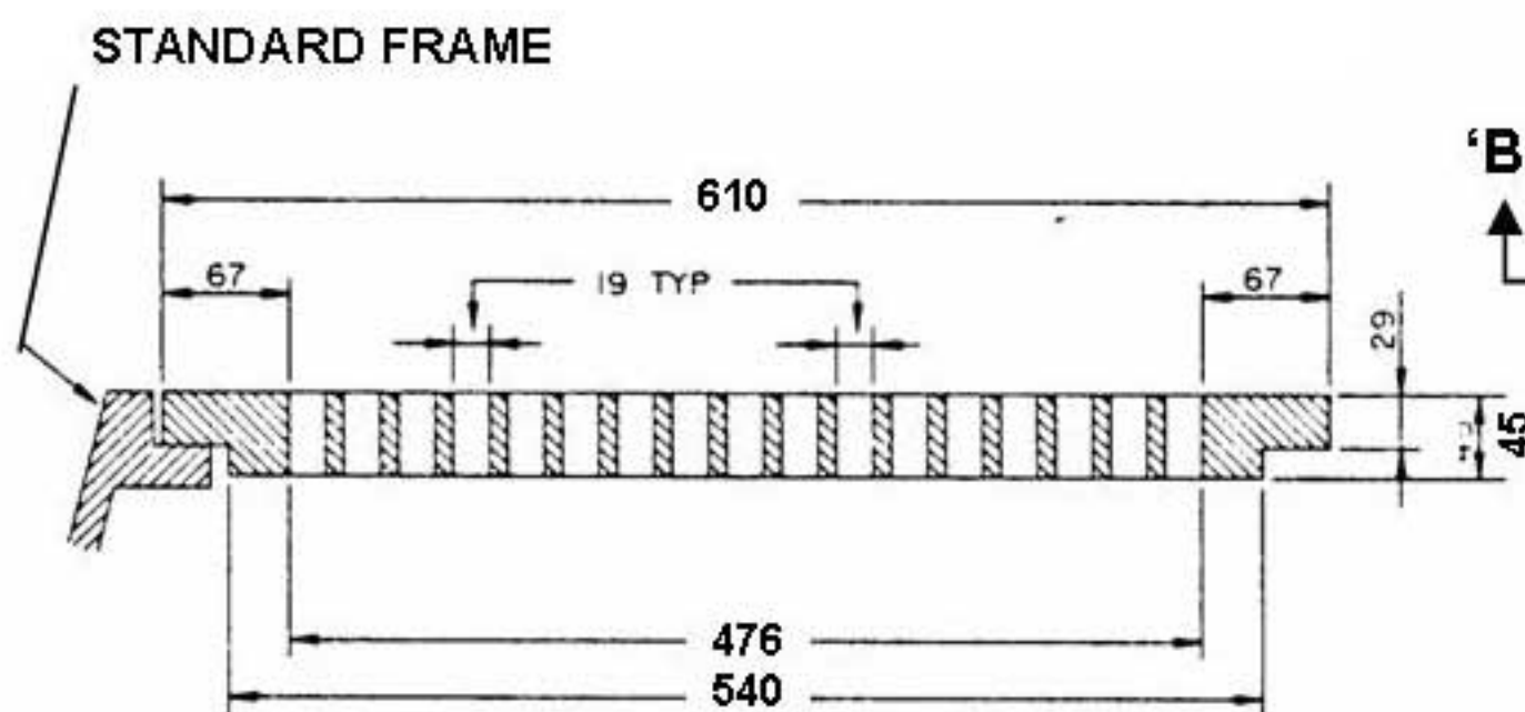
GRATE - SECTION 'B-B'
