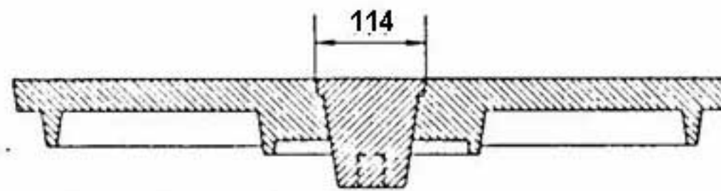
VALVE CHAMBER COVER AND PLUG
