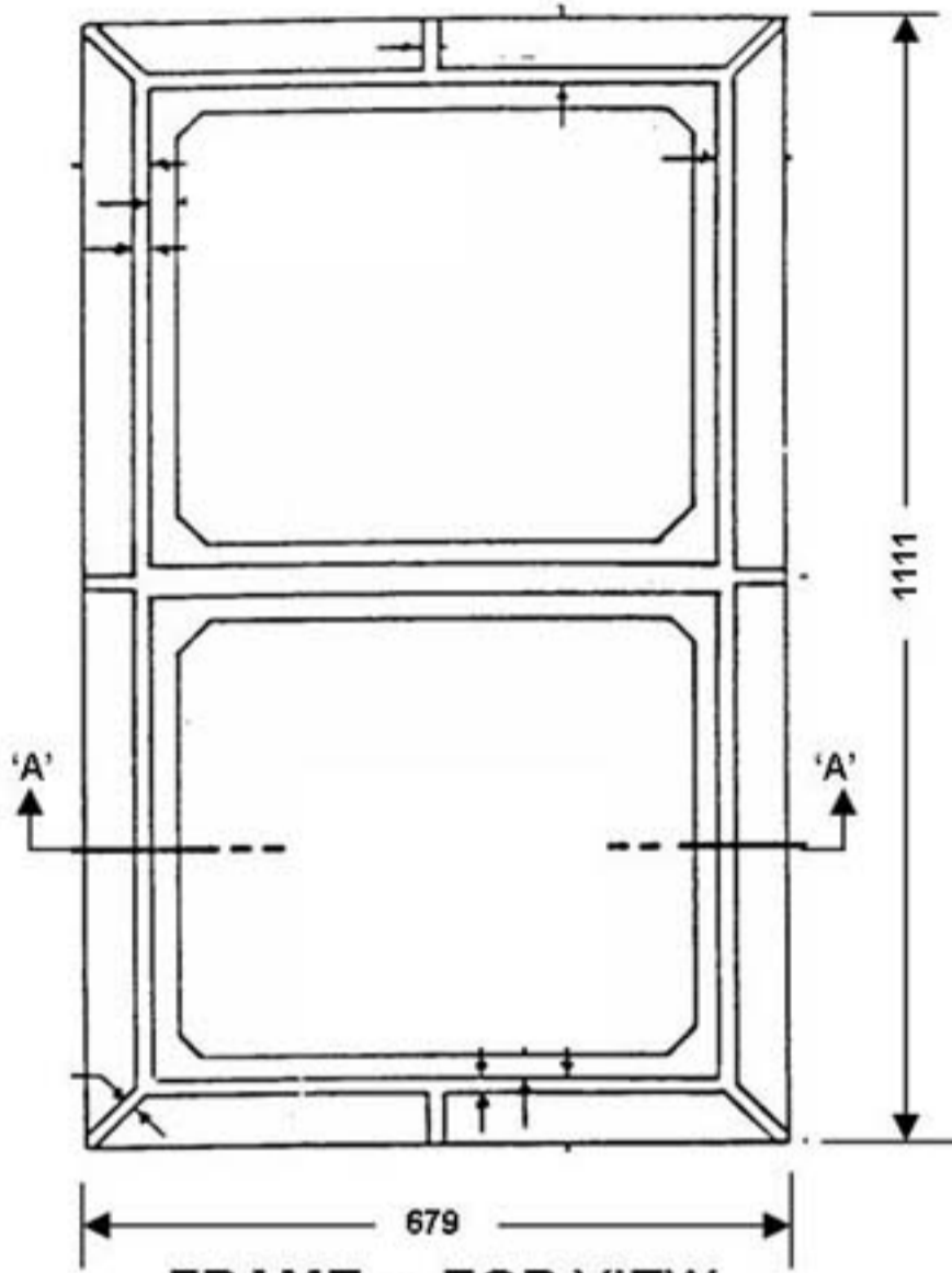
FRAME - TOP VIEW
