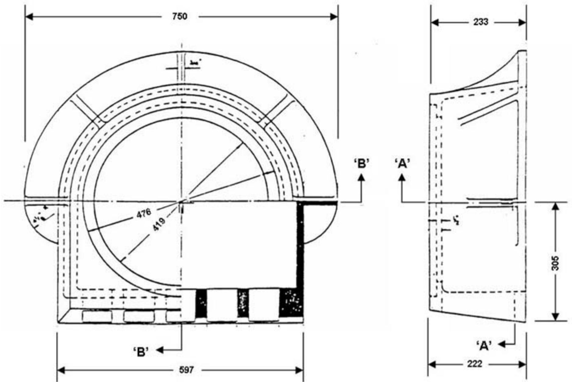
FRAME - TOP VIEW AND SECTION 'A-A'
