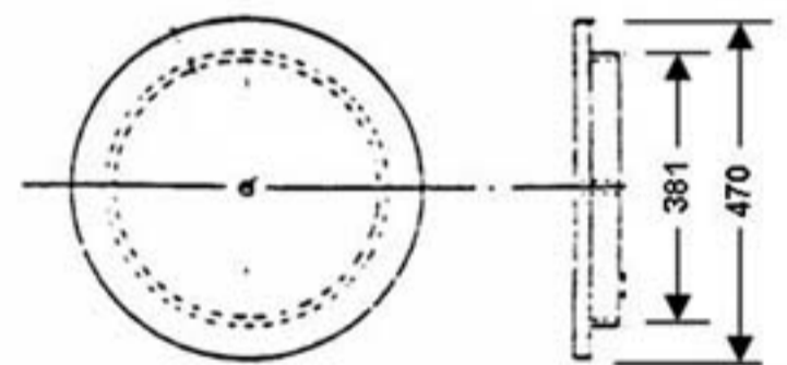
COVER - TOP & SIDE VIEW
